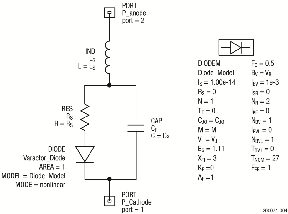
Figure 4. SPICE Model
